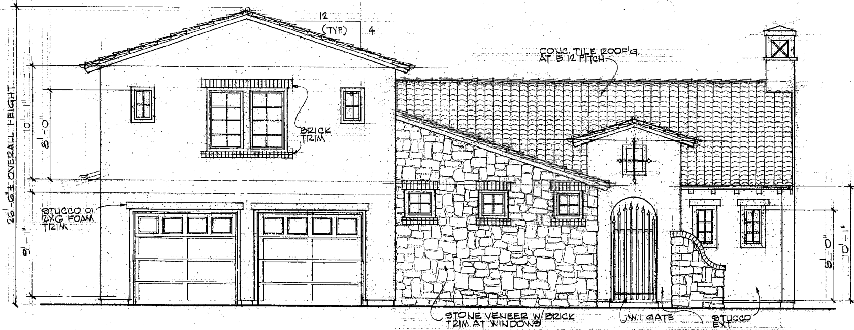
EAST ELEVATION (FRONT) SCALE: 1/4" = 1'-0"
