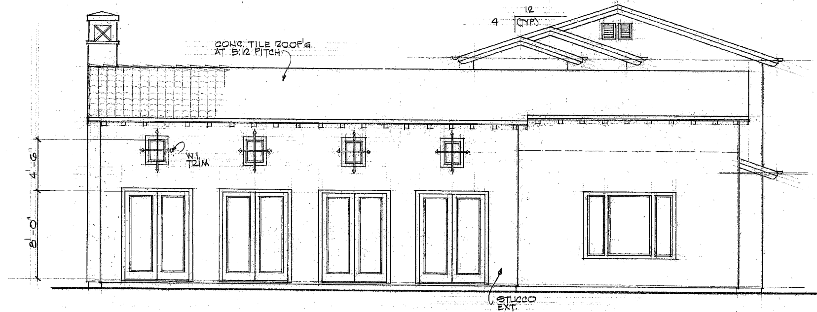
WEST ELEVATION (REAR) SCALE: 1/4" = 1'-0"
