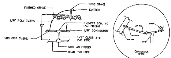
RISER TO DRIP TUBING DETAIL NOT TO SCALE
