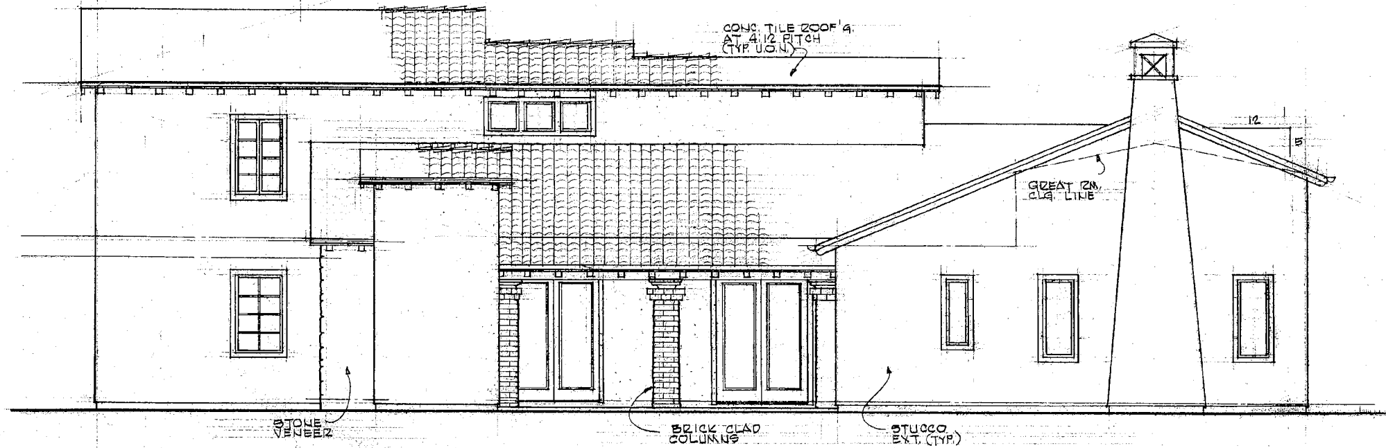
NORTH ELEVATION (RIGHT SIDE) SCALE: 1/4" = 1'-0"
