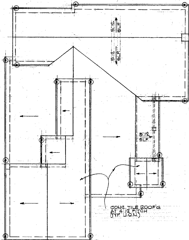
ROOF PLAN SCALE: 1/8" = 1'-0"
