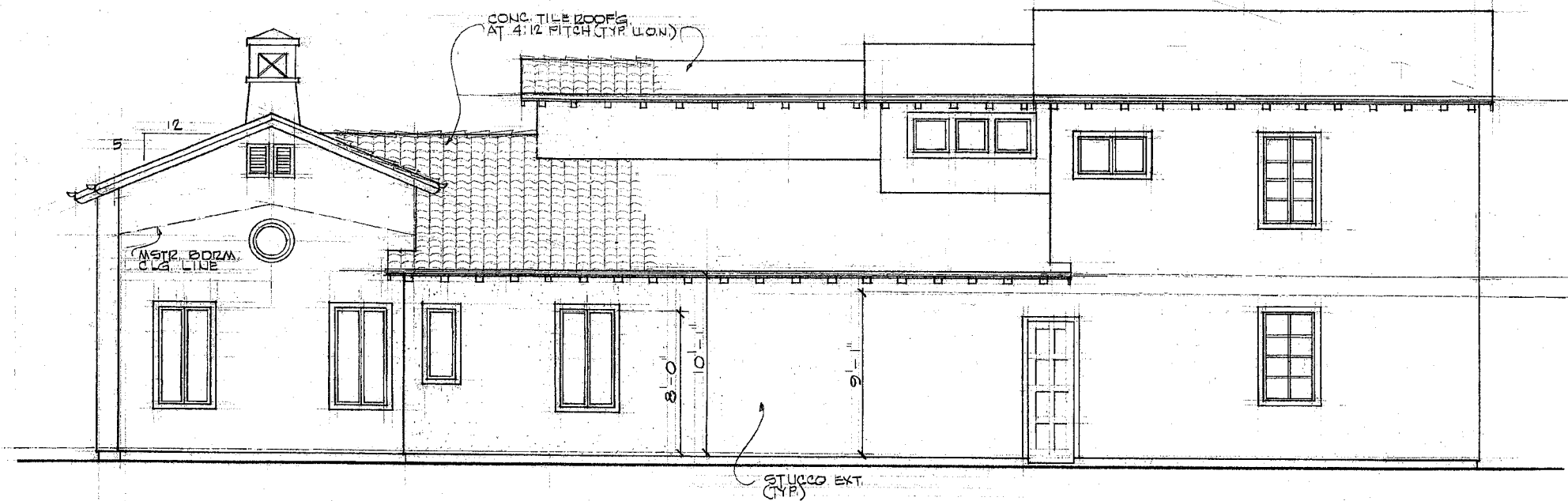
SOUTH ELEVATION (LEFT SIDE) SCALE: 1/4" = 1'-0"
