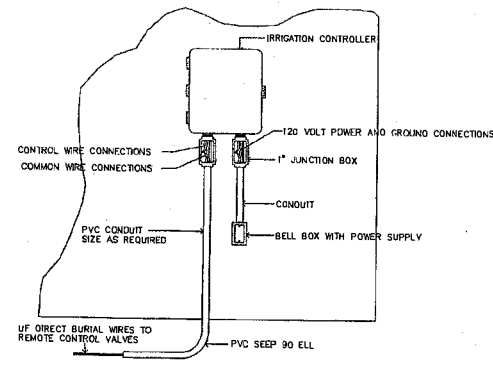
WALL MOUNT AUTOMATIC CONTROLLER NOT TO SCALE
