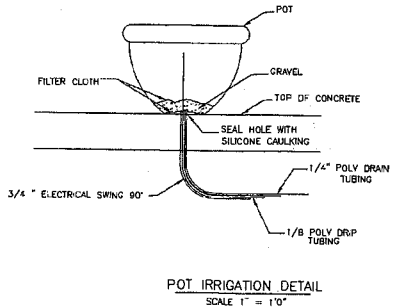
POT IRRIGATION DETAIL SCALE 1" = 10"
