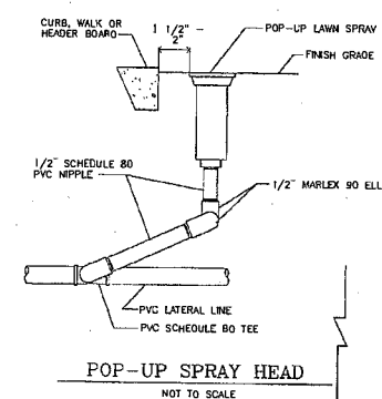
POP-UP SPRAY HEAD NOT TO SCALE
