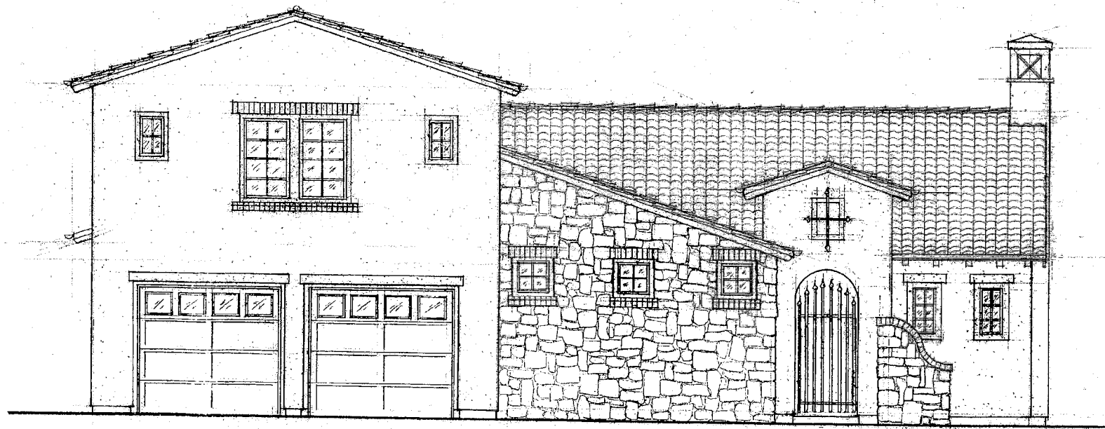
EAST ELEVATION (FRONT) SCALE: 1/4" = 1'-0"
