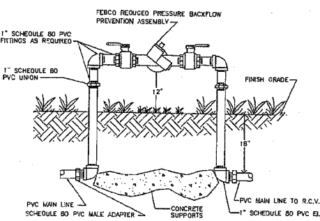
REDUCED PRESSURE BACKFLOW ASSEMBLY NOT TO SCALE
