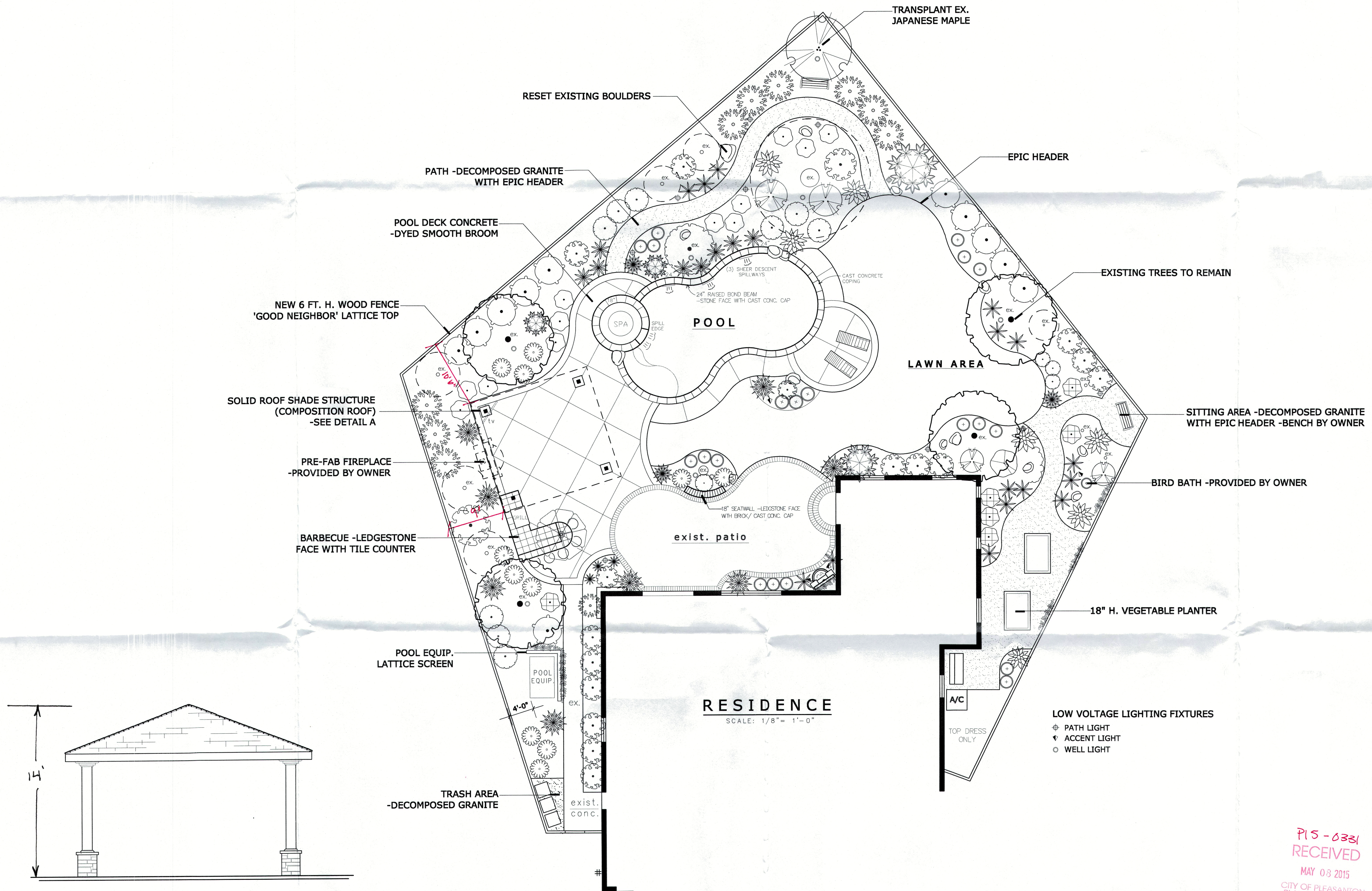
A SOLID ROOF SHADE STRUCTURE CONCEPT ELEVATION
