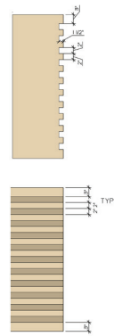
PRECAST PANEL WITH HORIZONTAL REVEALS
